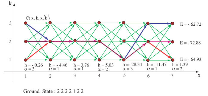
Fig. 18. The graph corresponding to the Shortest Path Method for the RFPC problem.
